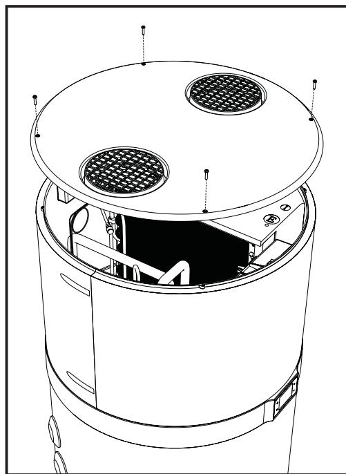
fig. 41 - Top cover removal
