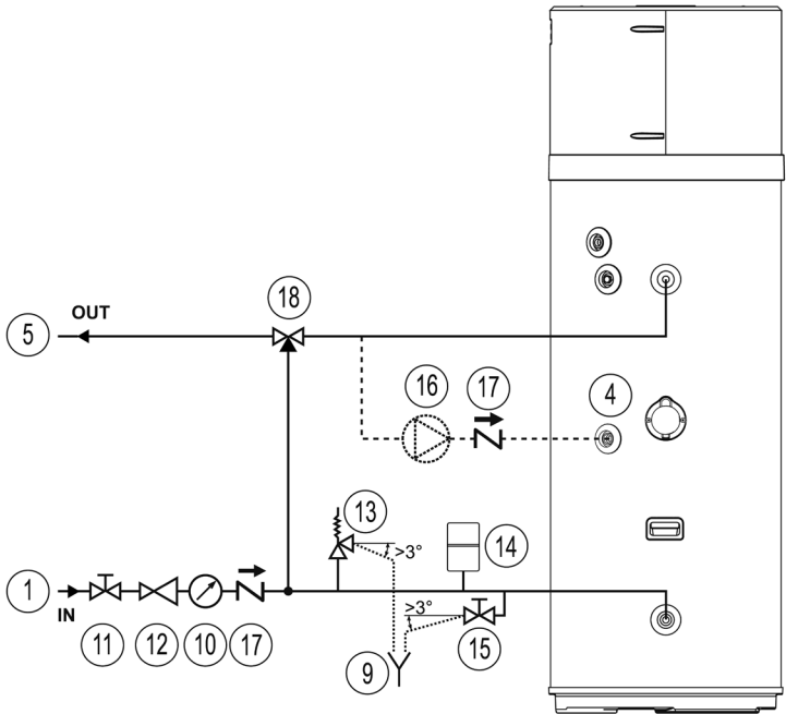
fig. 16 - Example of water system
