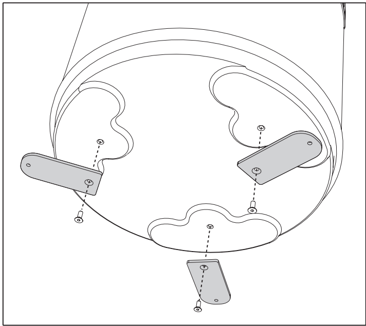
fig. 10 - Fastening brackets
