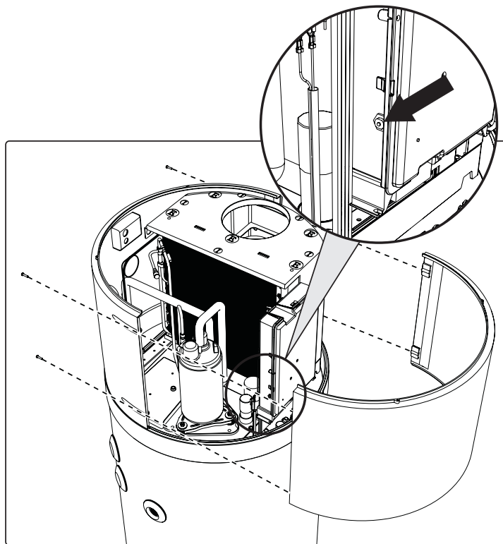
fig. 42 - Front panel removal
